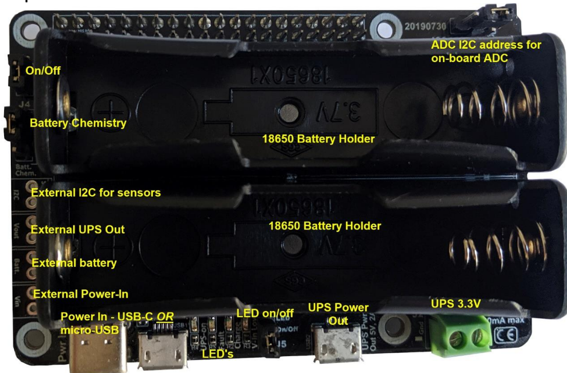
Pi-Z-UpTime UPS 2.0
